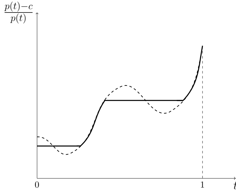
Figure 3: Mark-up for the relaxed solution (dashed line) and for the complete solution (solid line), with c > 0 .
